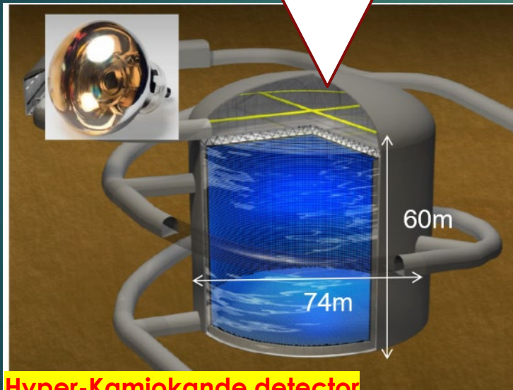
Hyper-Kamiokande detector
